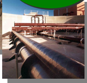
SBR FLOW CONTROL AND SBR JET
